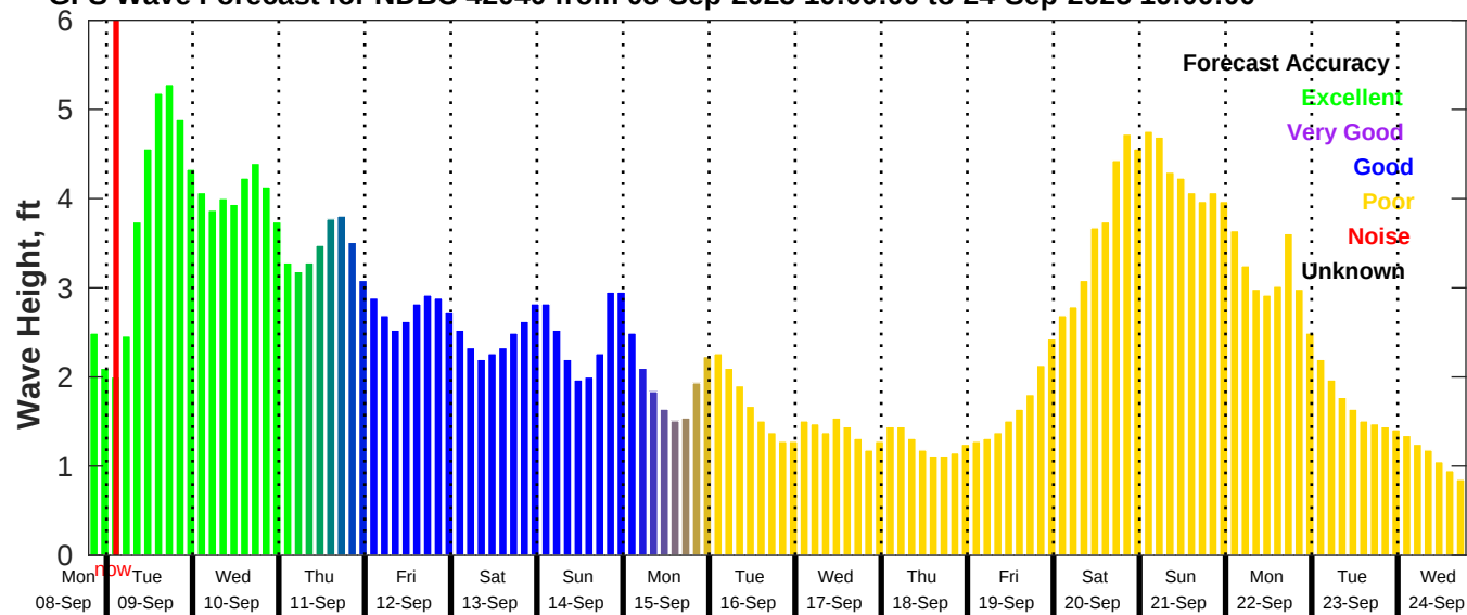
GFS Wave Forecast for NDBC 42040 from 08-Sep-2025 19:00:00 to 24-Sep-2025 19:00:00
