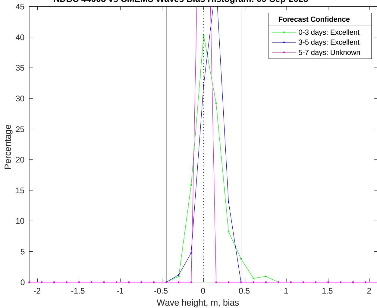
NDBC 44008 vs CMEMS Waves Bias Histogram: 09-Sep-2025
