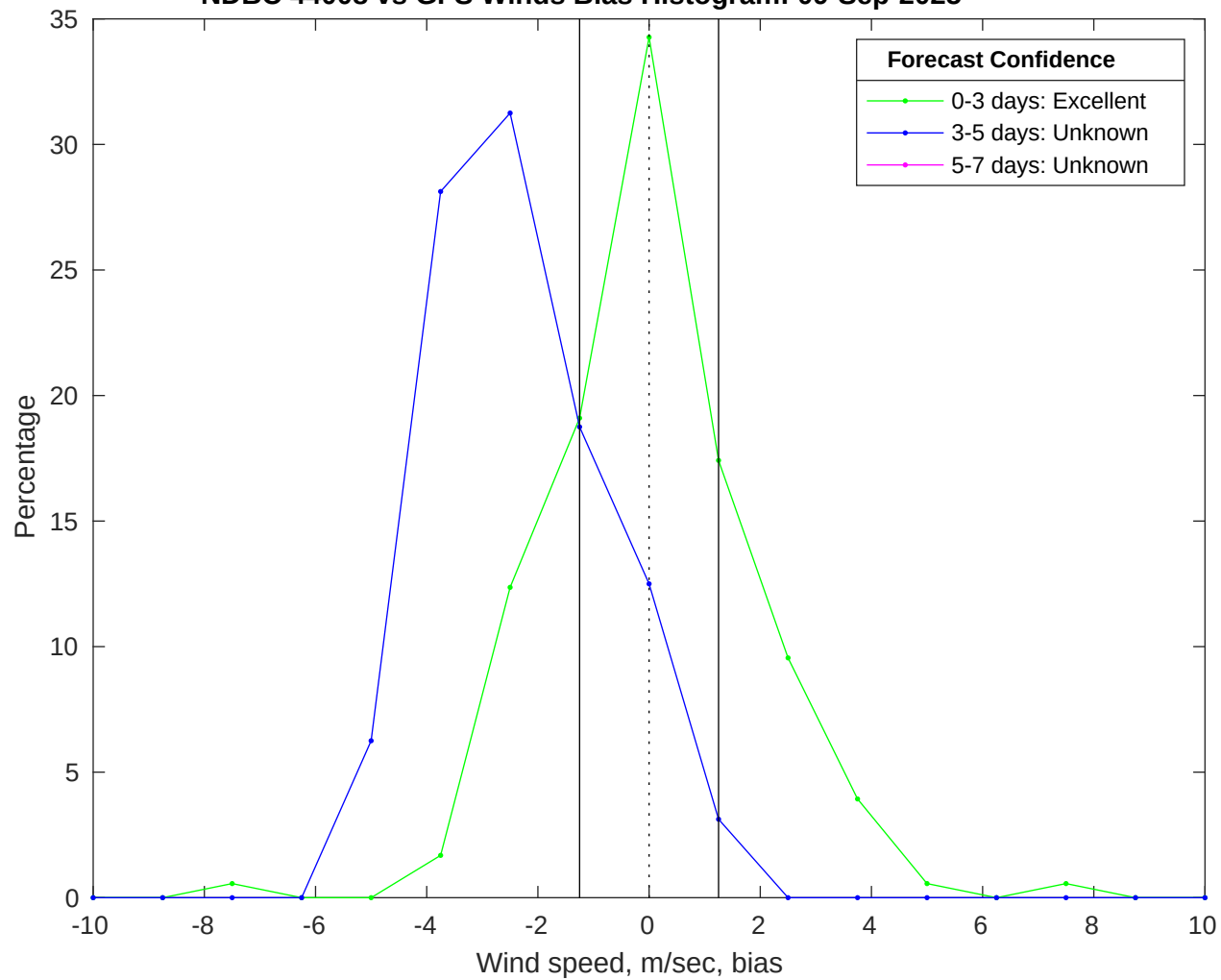
NDBC 44008 vs GFS Winds Bias Histogram: 09-Sep-2025
