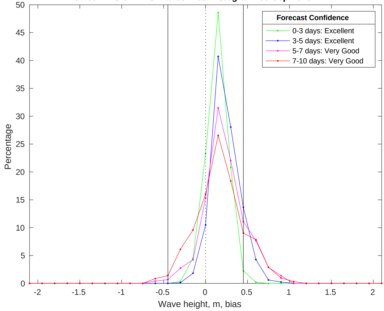
NDBC 46011 vs CMEMS Waves Bias Histogram: 09-Sep-2025
