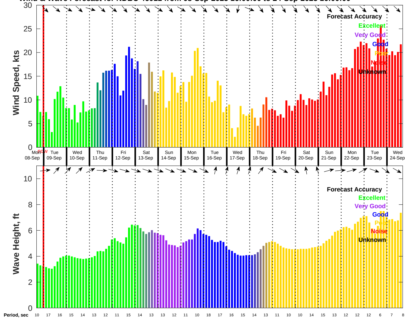
Wind & Wave Forecast for NDBC 46011 from 08-Sep-2025 16:00:00 to 24-Sep-2025 16:00:00
