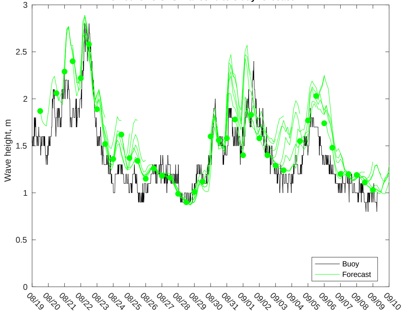
NDBC 46028 vs GFS Waves: 0 to 3 day forecast
