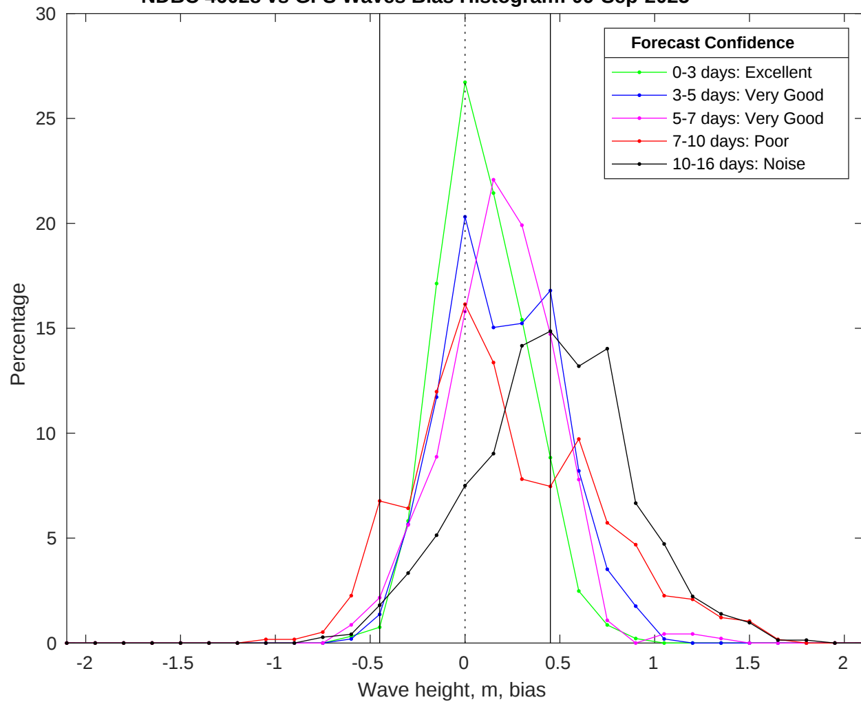
NDBC 46028 vs GFS Waves Bias Histogram: 09-Sep-2025
