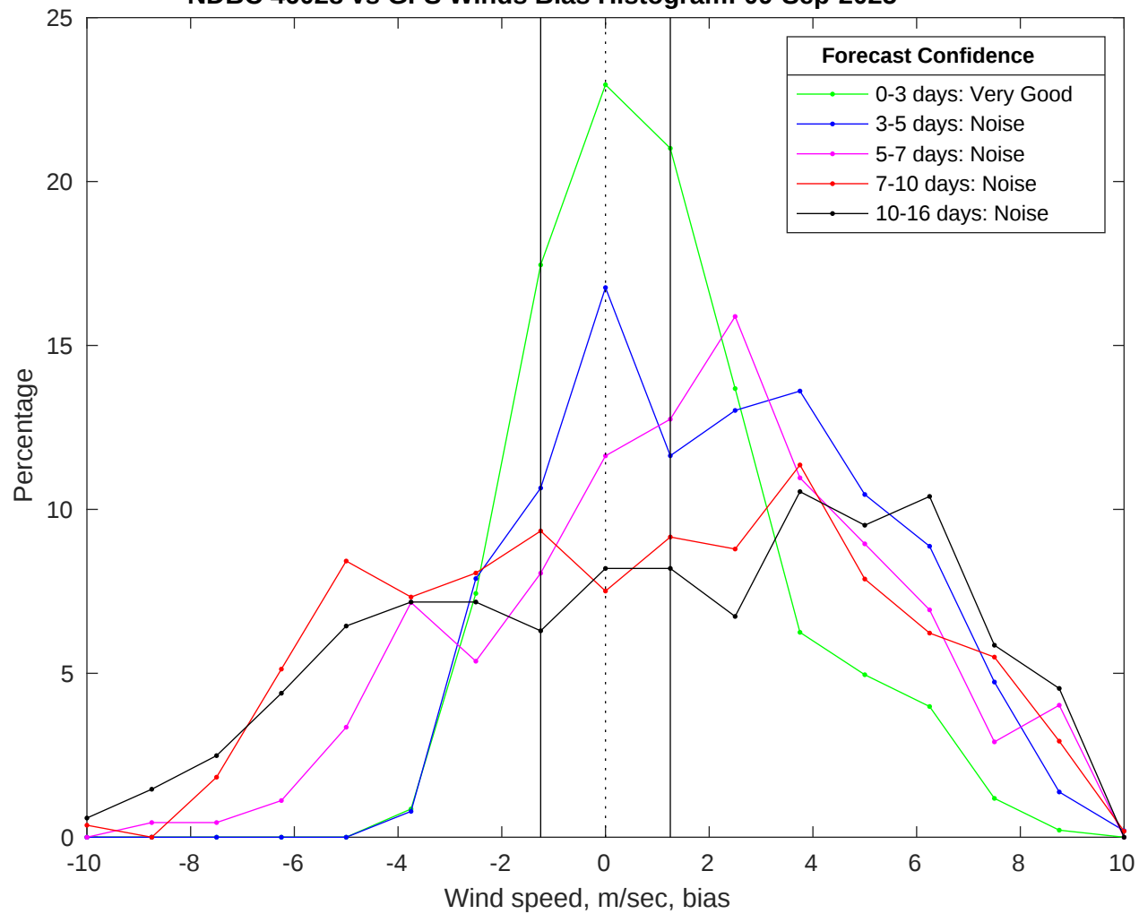
NDBC 46028 vs GFS Winds Bias Histogram: 09-Sep-2025
