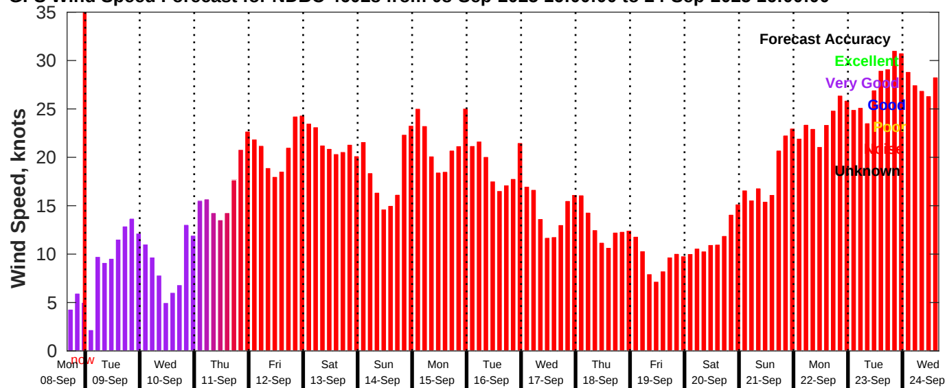
GFS Wind Speed Forecast for NDBC 46028 from 08-Sep-2025 16:00:00 to 24-Sep-2025 16:00:00
