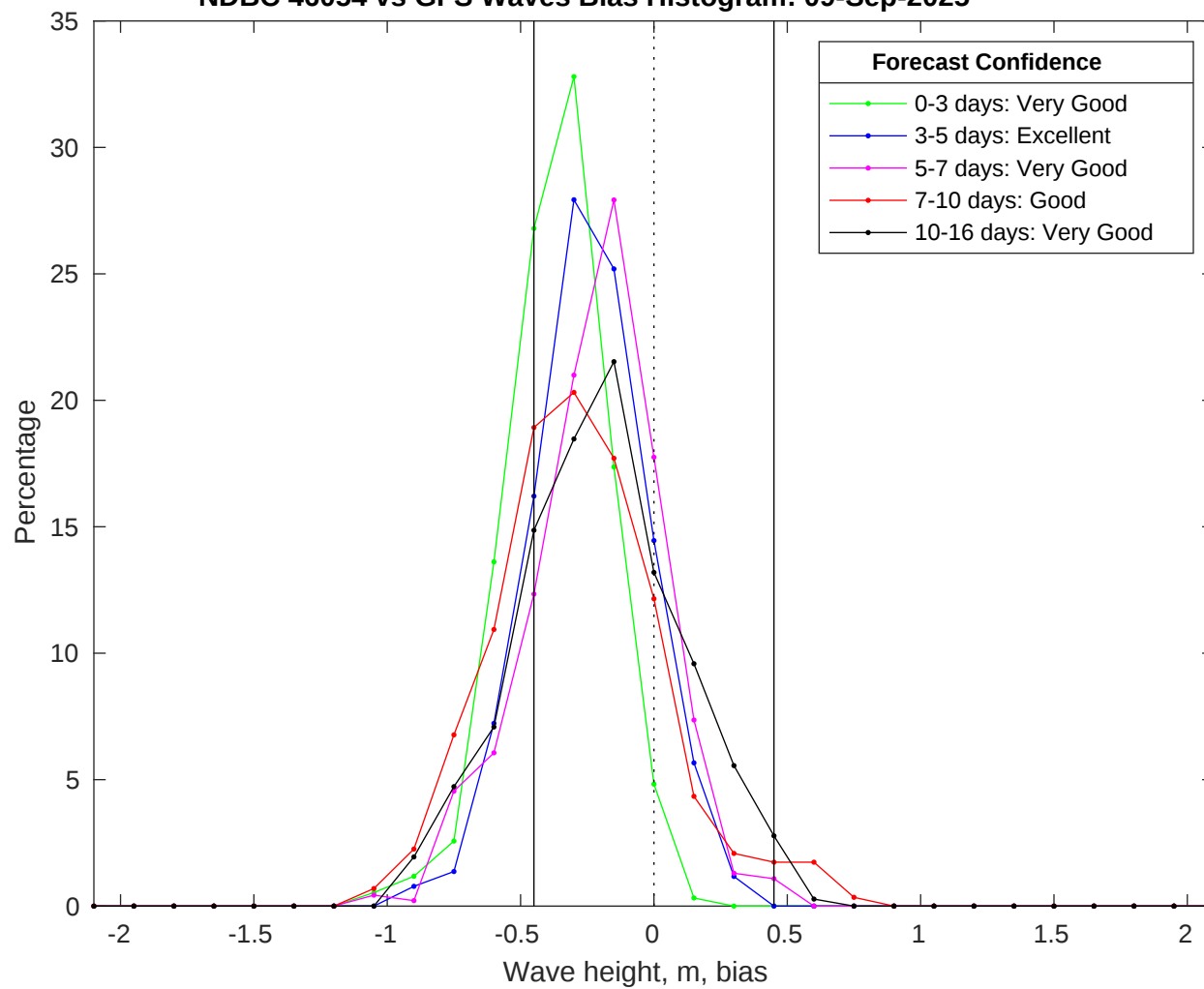
NDBC 46054 vs GFS Waves Bias Histogram: 09-Sep-2025
