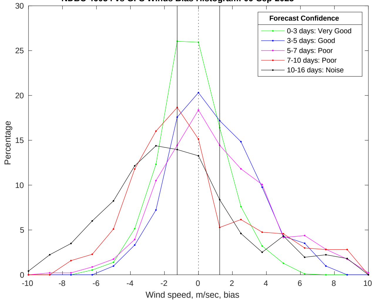
NDBC 46054 vs GFS Winds Bias Histogram: 09-Sep-2025
