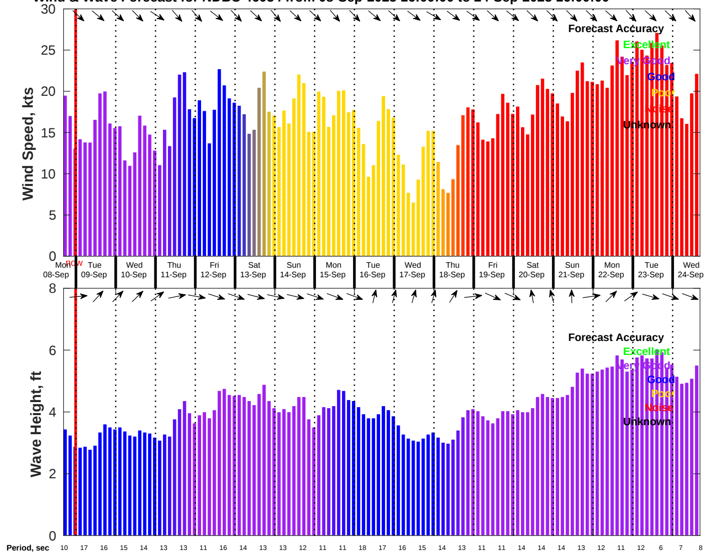
Wind & Wave Forecast for NDBC 46054 from 08-Sep-2025 16:00:00 to 24-Sep-2025 16:00:00
