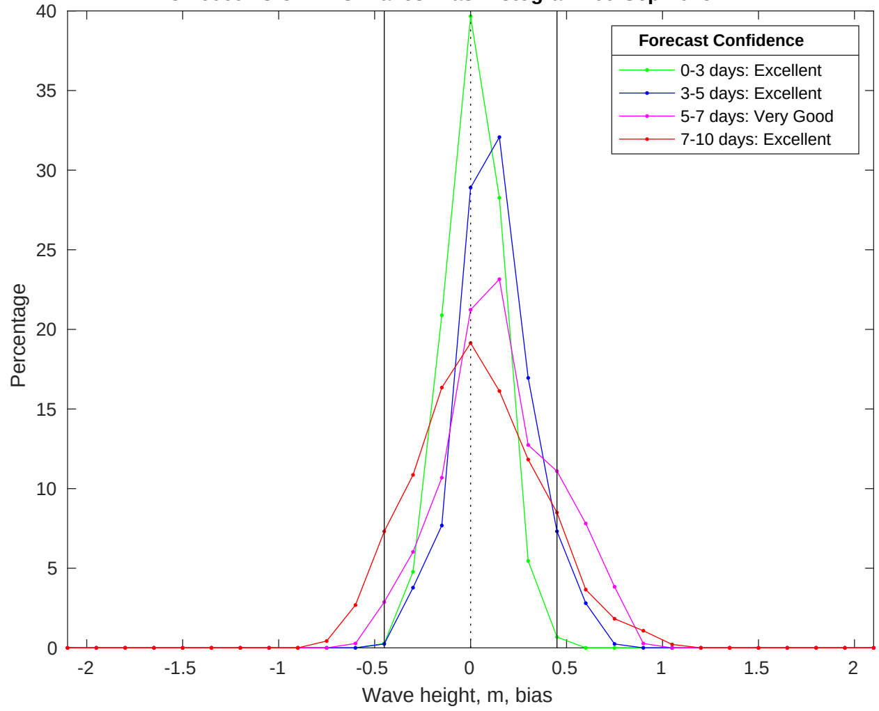
NDBC 46069 vs CMEMS Waves Bias Histogram: 09-Sep-2025
