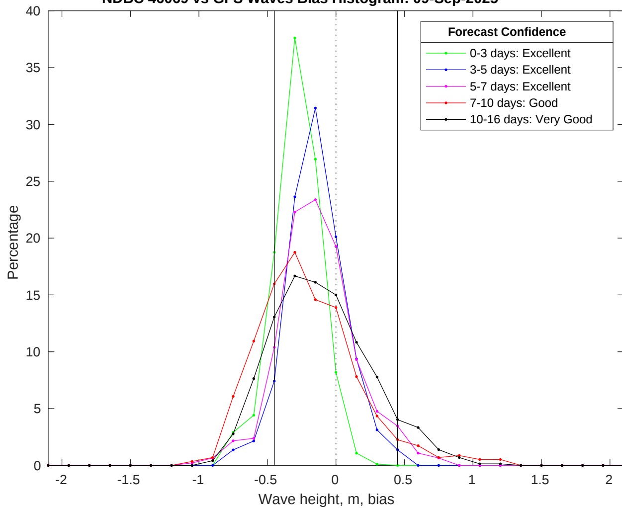
NDBC 46069 vs GFS Waves Bias Histogram: 09-Sep-2025
