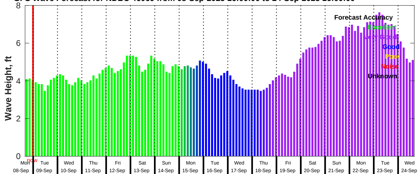
GFS Wave Forecast for NDBC 46069 from 08-Sep-2025 16:00:00 to 24-Sep-2025 16:00:00
