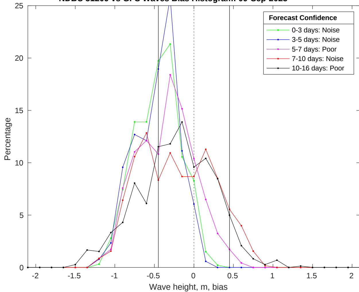
NDBC 51209 vs GFS Waves Bias Histogram: 09-Sep-2025
