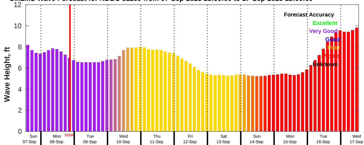
CMEMS Wave Forecast for NDBC 51209 from 07-Sep-2025 13:00:00 to 17-Sep-2025 13:00:00
