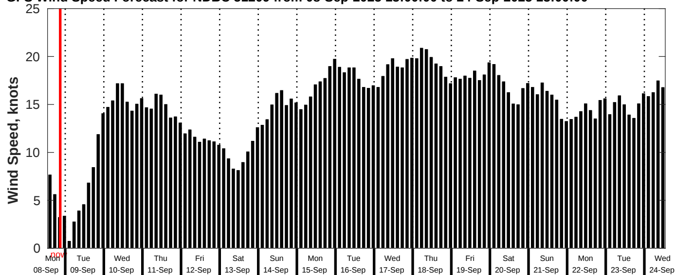
GFS Wind Speed Forecast for NDBC 51209 from 08-Sep-2025 13:00:00 to 24-Sep-2025 13:00:00
