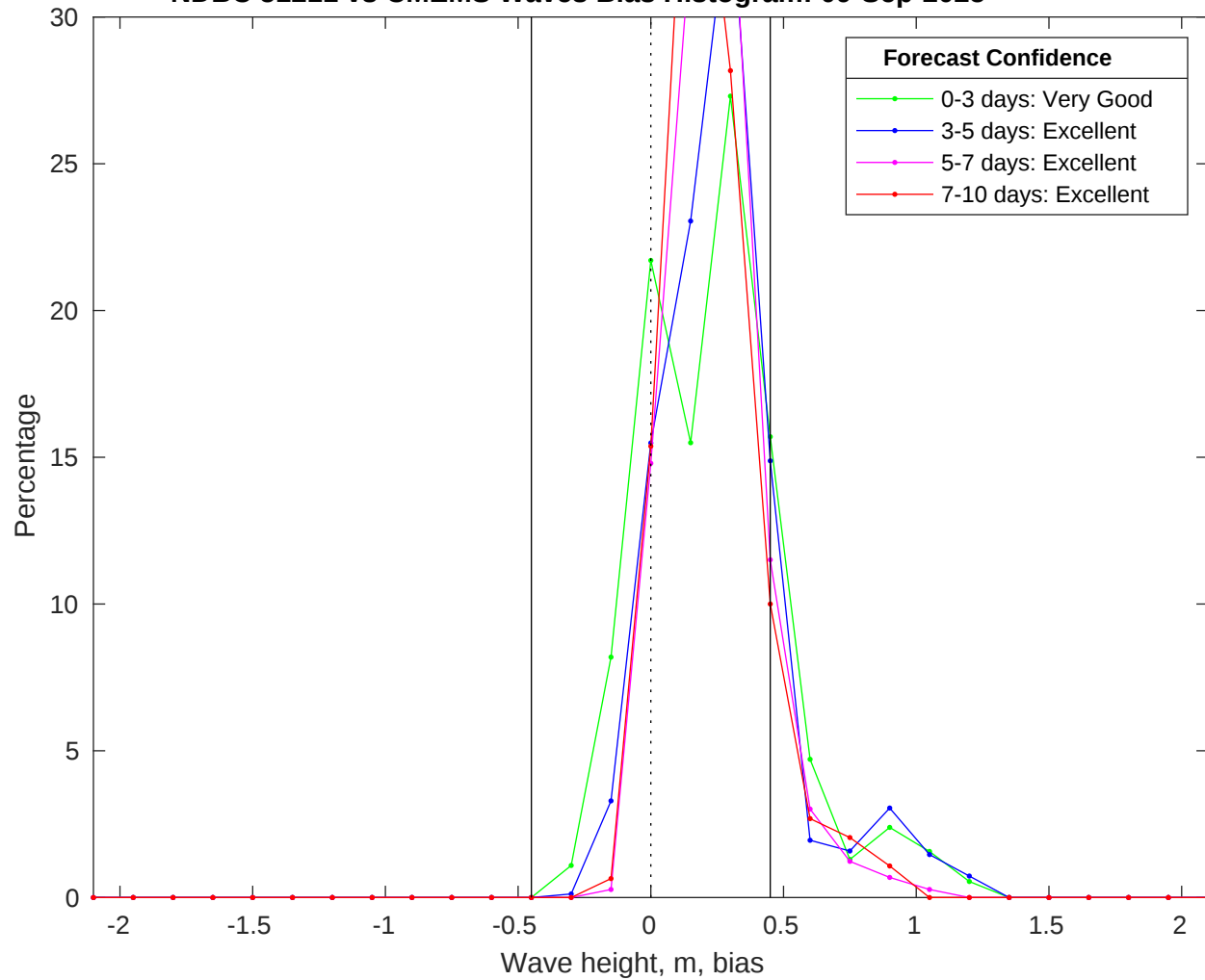
NDBC 51211 vs CMEMS Waves Bias Histogram: 09-Sep-2025
