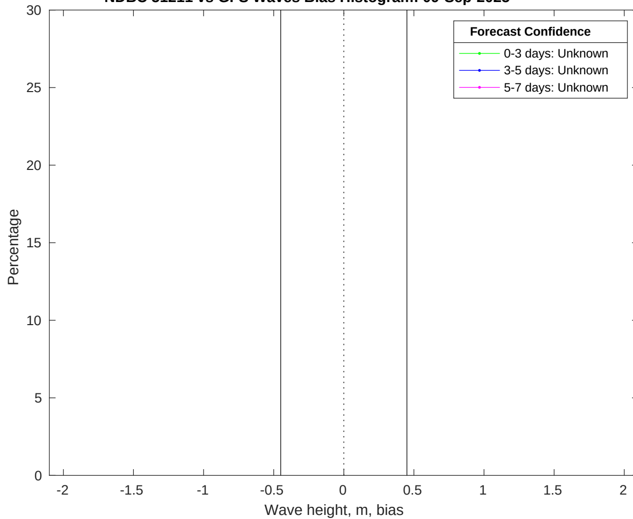
NDBC 51211 vs GFS Waves Bias Histogram: 09-Sep-2025
