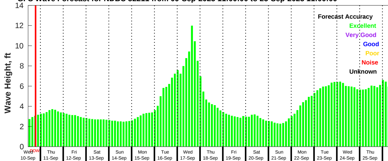
GFS Wave Forecast for NDBC 52211 from 09-Sep-2025 11:00:00 to 25-Sep-2025 11:00:00
