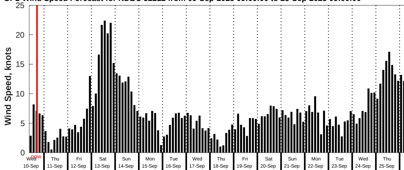
GFS Wind Speed Forecast for NDBC 52212 from 09-Sep-2025 09:00:00 to 25-Sep-2025 09:00:00
