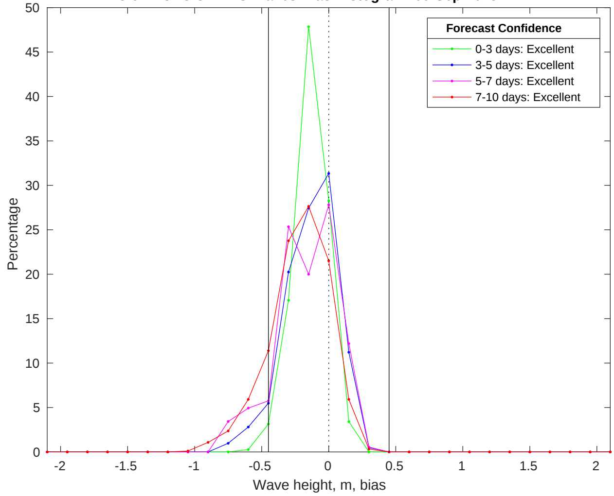
NDBC 52213 vs CMEMS Waves Bias Histogram: 09-Sep-2025
