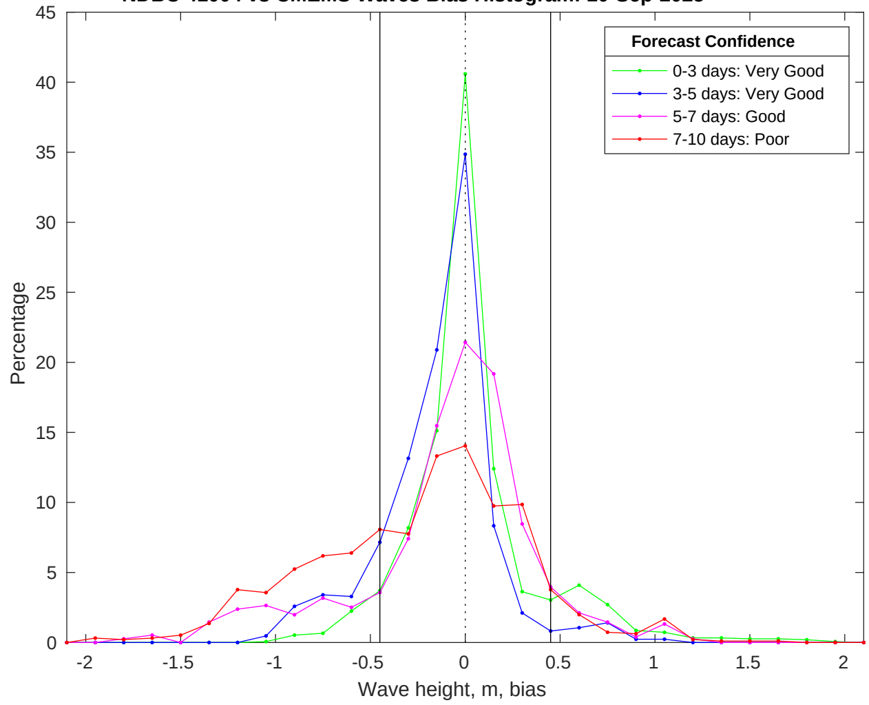
NDBC 41004 vs CMEMS Waves Bias Histogram: 10-Sep-2025
