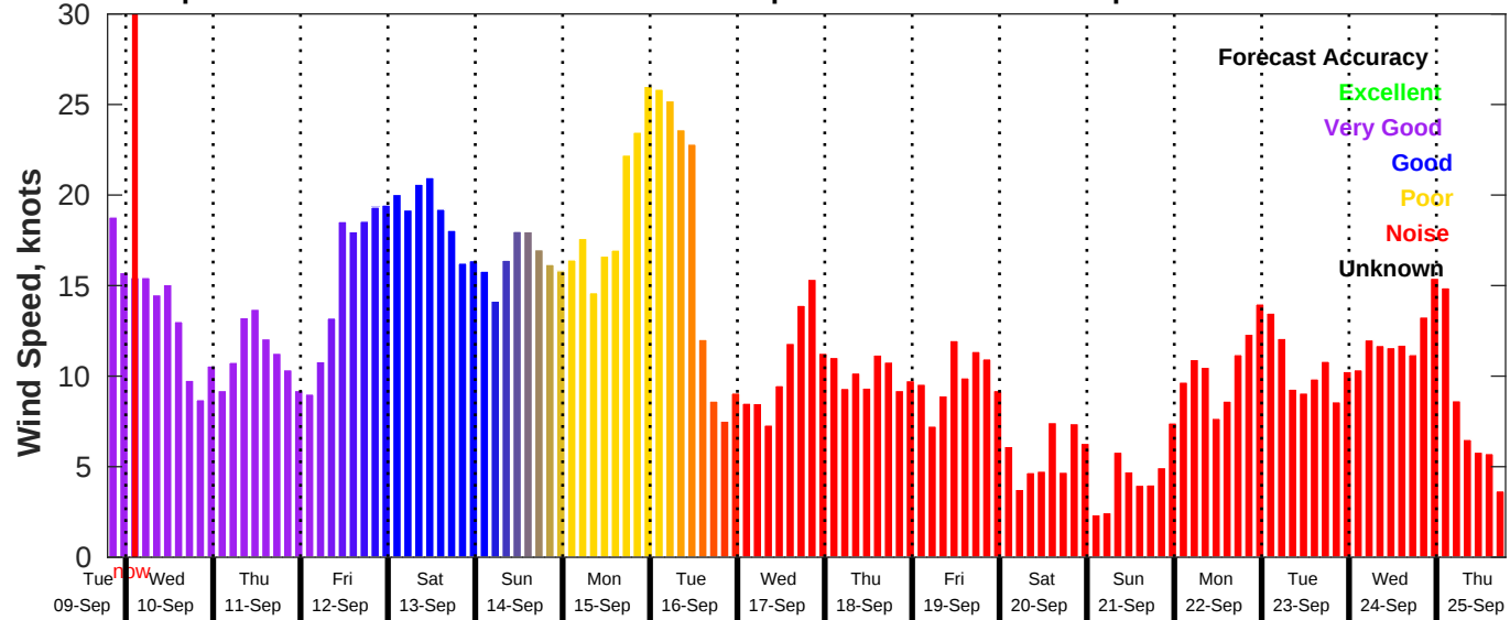
GFS Wind Speed Forecast for NDBC 41004 from 09-Sep-2025 19:00:00 to 25-Sep-2025 19:00:00
