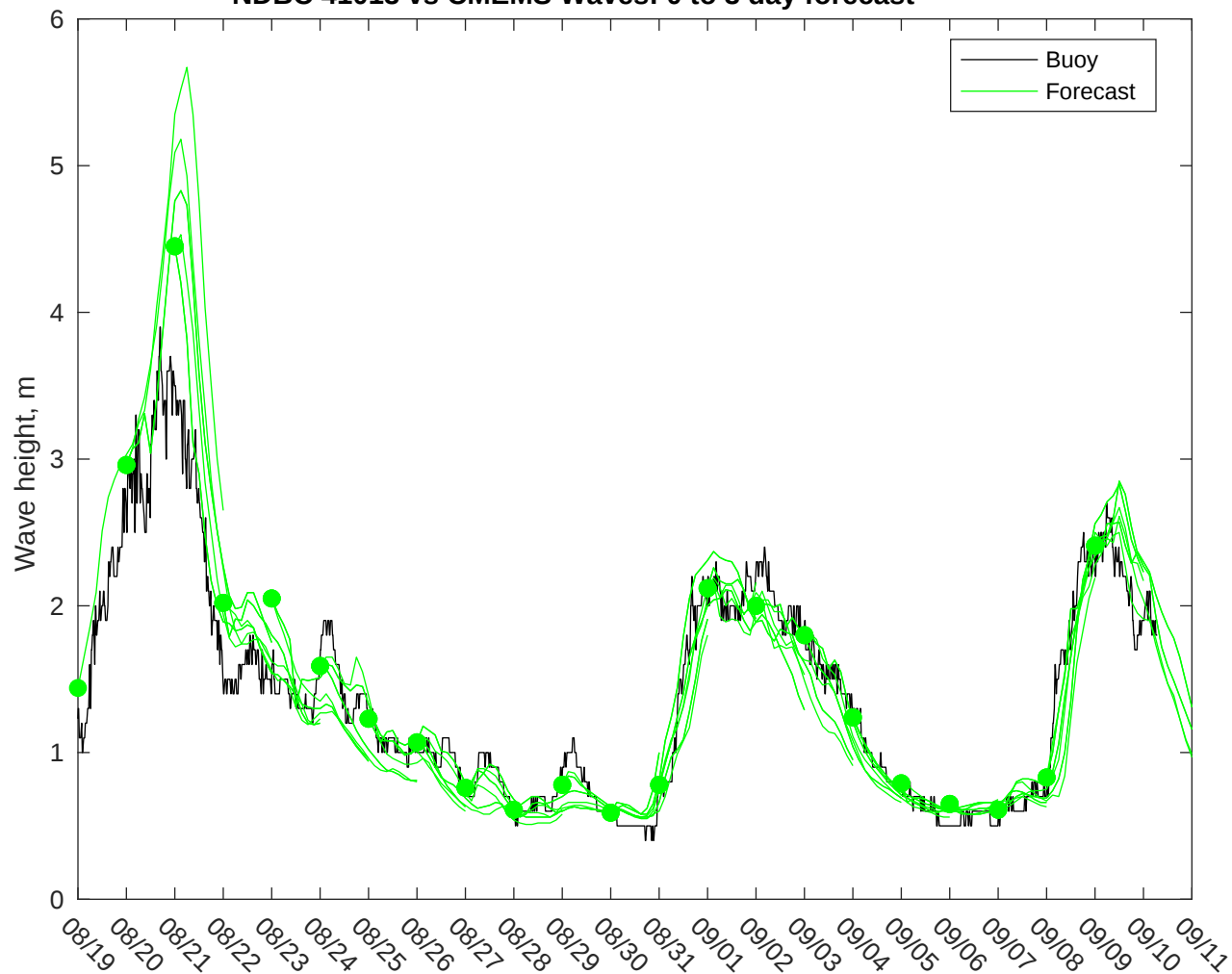
NDBC 41013 vs CMEMS Waves: 0 to 3 day forecast
