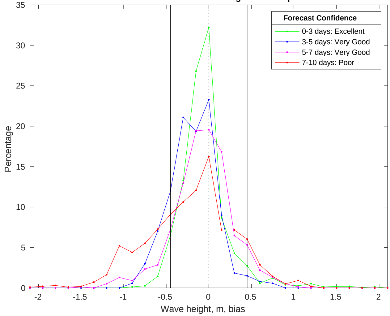
NDBC 41013 vs CMEMS Waves Bias Histogram: 10-Sep-2025
