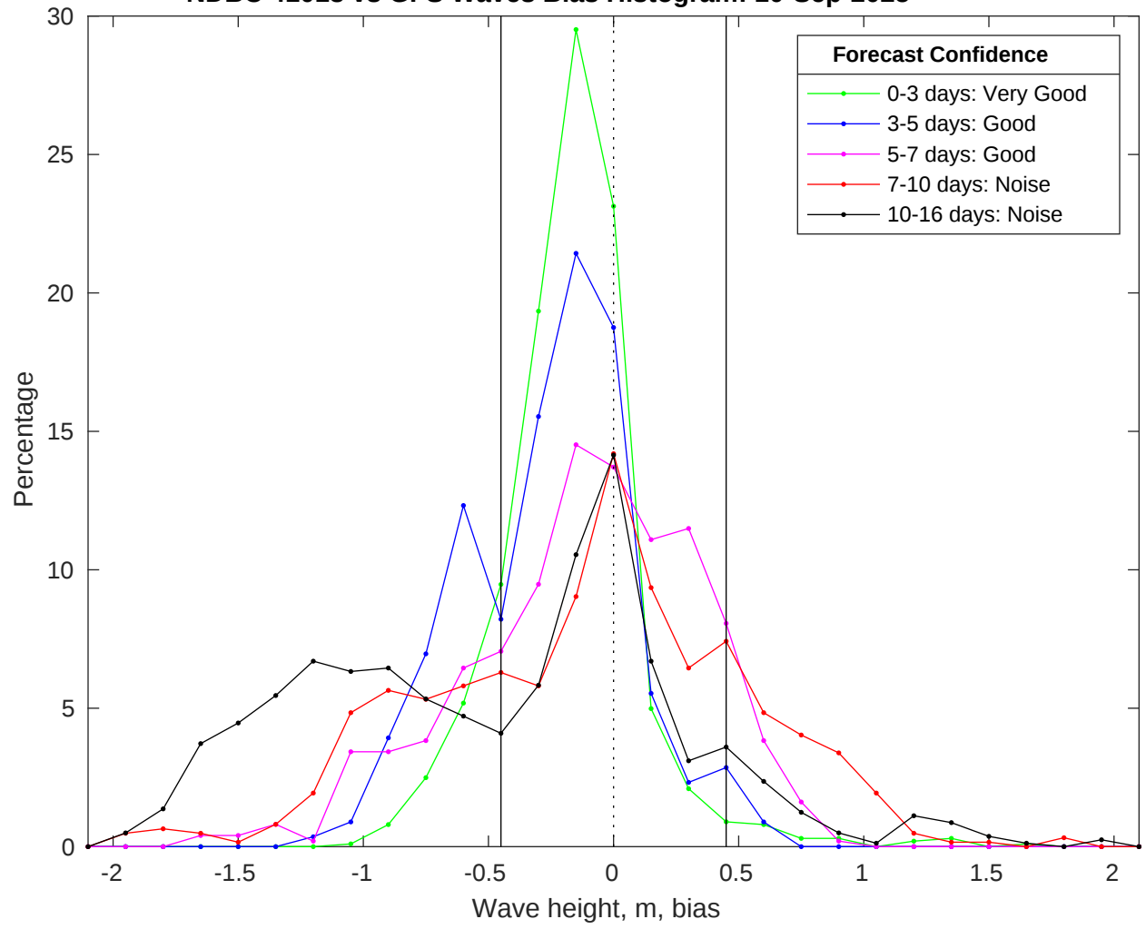
NDBC 41013 vs GFS Waves Bias Histogram: 10-Sep-2025
