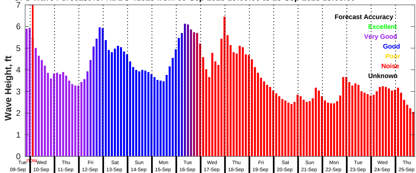
GFS Wave Forecast for NDBC 41013 from 09-Sep-2025 19:00:00 to 25-Sep-2025 19:00:00
