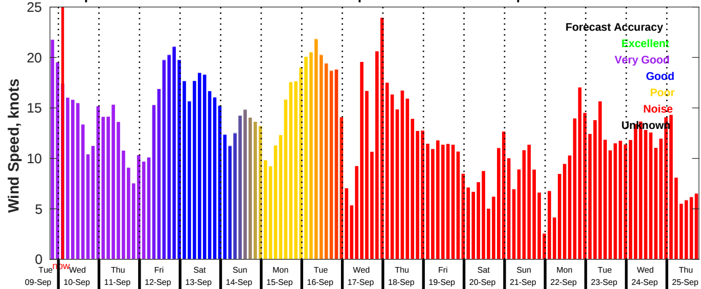
GFS Wind Speed Forecast for NDBC 41013 from 09-Sep-2025 19:00:00 to 25-Sep-2025 19:00:00
