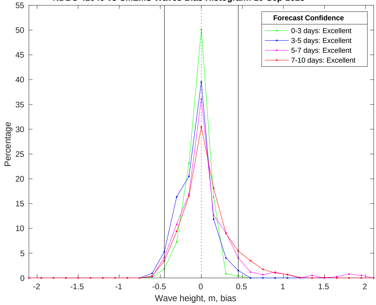
NDBC 41040 vs CMEMS Waves Bias Histogram: 10-Sep-2025
