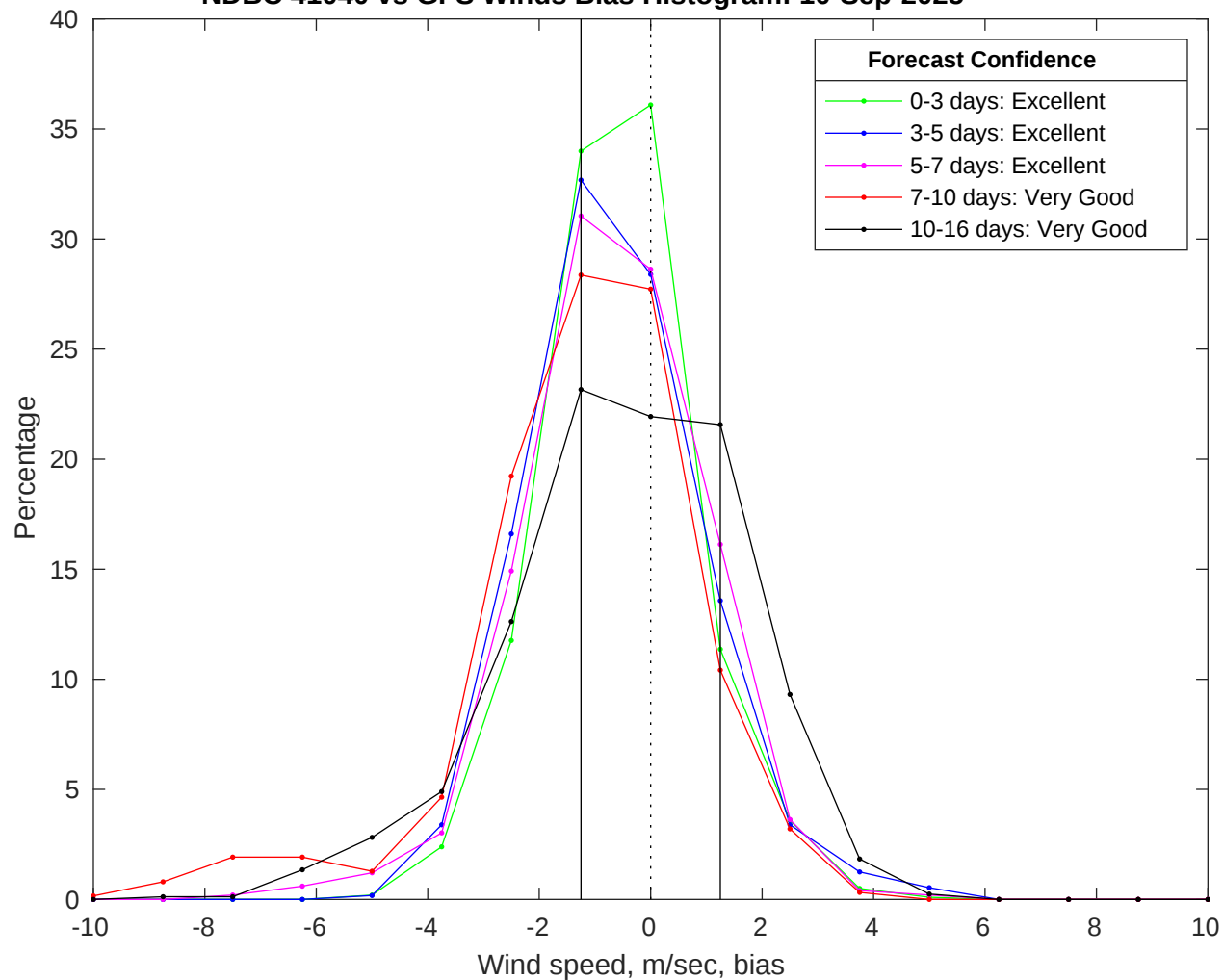
NDBC 41040 vs GFS Winds Bias Histogram: 10-Sep-2025
