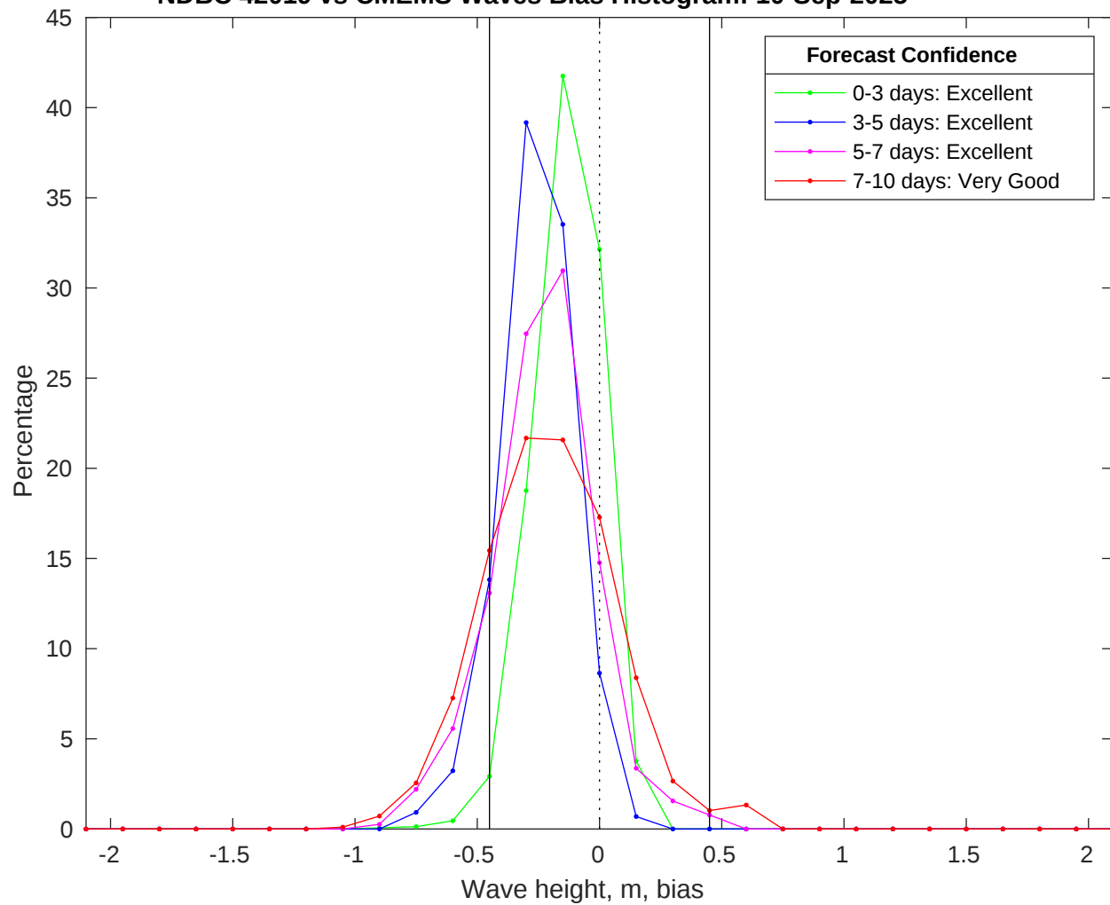
NDBC 42019 vs CMEMS Waves Bias Histogram: 10-Sep-2025
