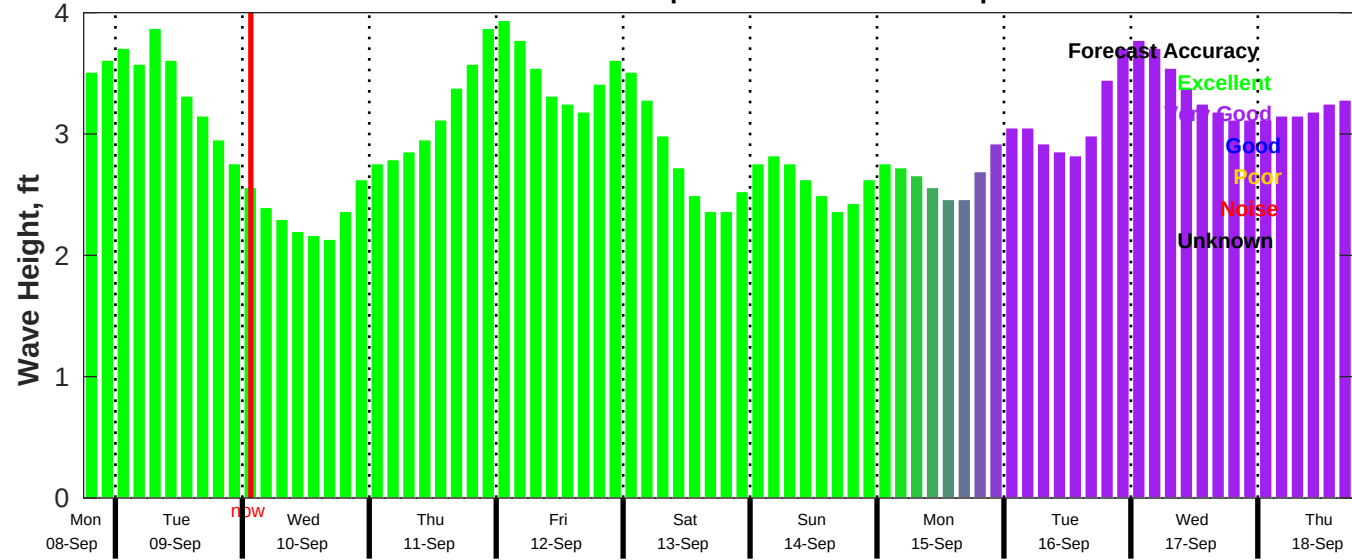
CMEMS Wave Forecast for NDBC 42019 from 08-Sep-2025 18:00:00 to 18-Sep-2025 18:00:00
