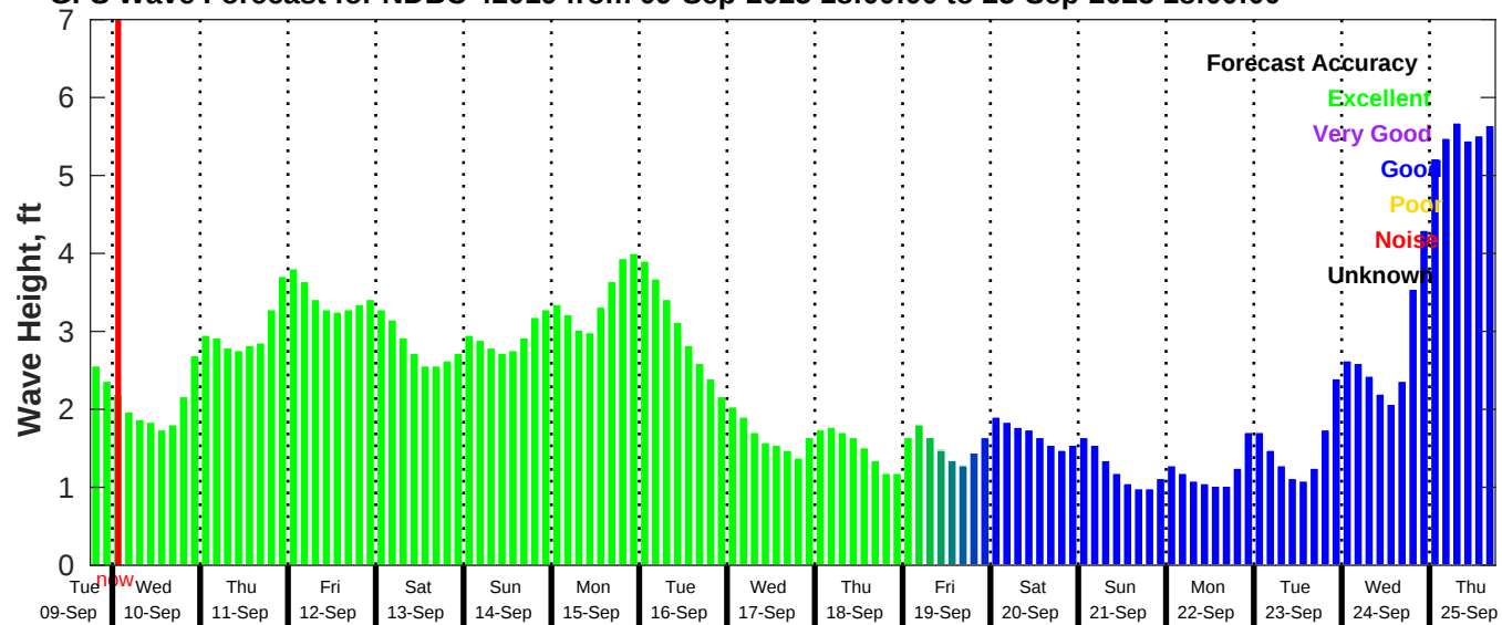
GFS Wave Forecast for NDBC 42019 from 09-Sep-2025 18:00:00 to 25-Sep-2025 18:00:00
