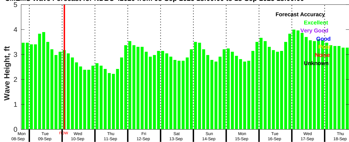
CMEMS Wave Forecast for NDBC 42020 from 08-Sep-2025 18:00:00 to 18-Sep-2025 18:00:00
