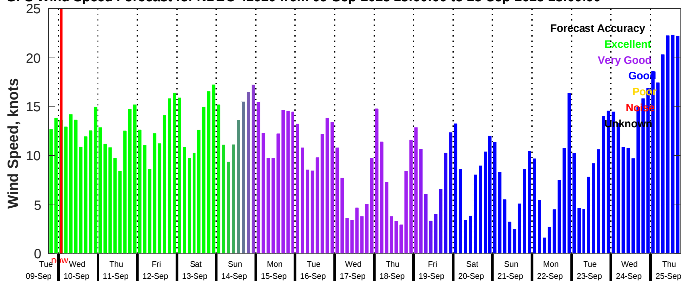
GFS Wind Speed Forecast for NDBC 42020 from 09-Sep-2025 18:00:00 to 25-Sep-2025 18:00:00
