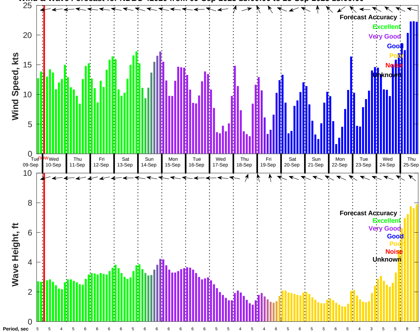
Wind & Wave Forecast for NDBC 42020 from 09-Sep-2025 18:00:00 to 25-Sep-2025 18:00:00
