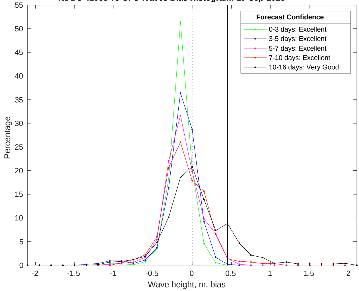
NDBC 42035 vs GFS Waves Bias Histogram: 10-Sep-2025
