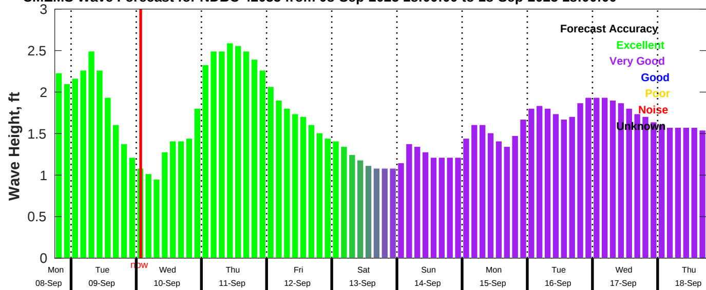
CMEMS Wave Forecast for NDBC 42035 from 08-Sep-2025 18:00:00 to 18-Sep-2025 18:00:00
