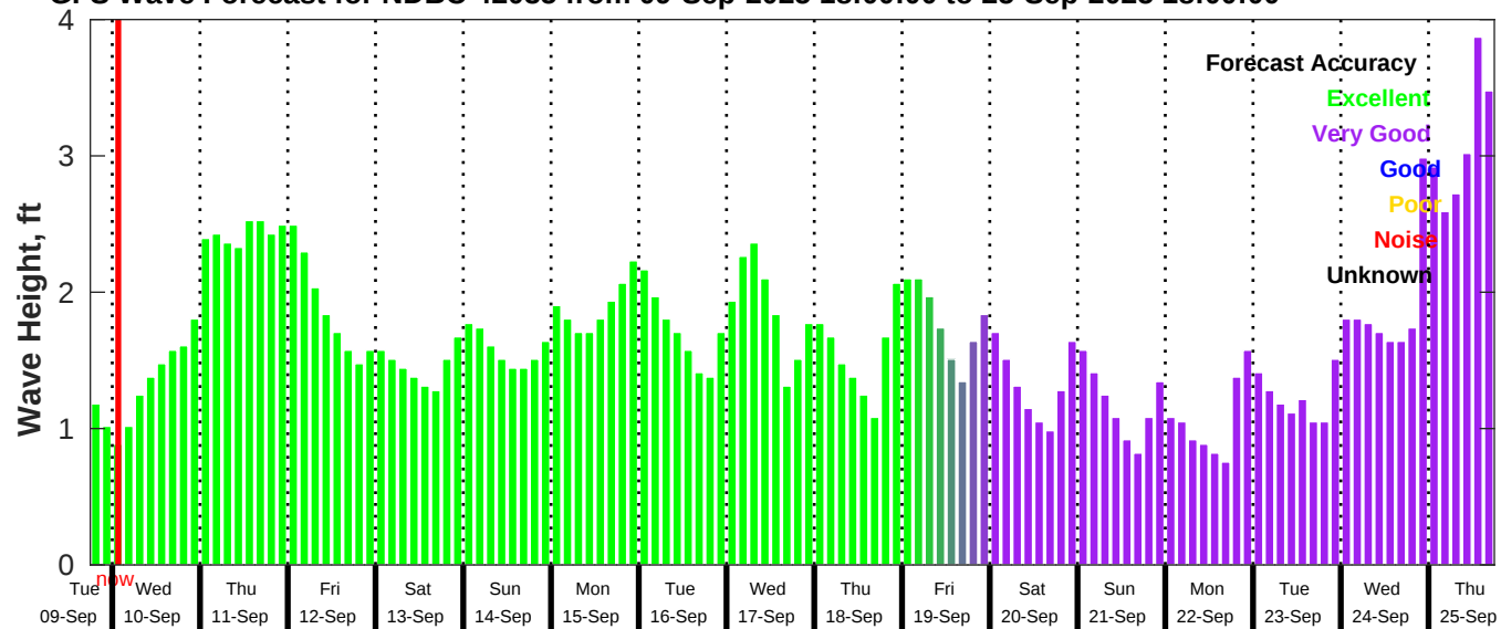
GFS Wave Forecast for NDBC 42035 from 09-Sep-2025 18:00:00 to 25-Sep-2025 18:00:00
