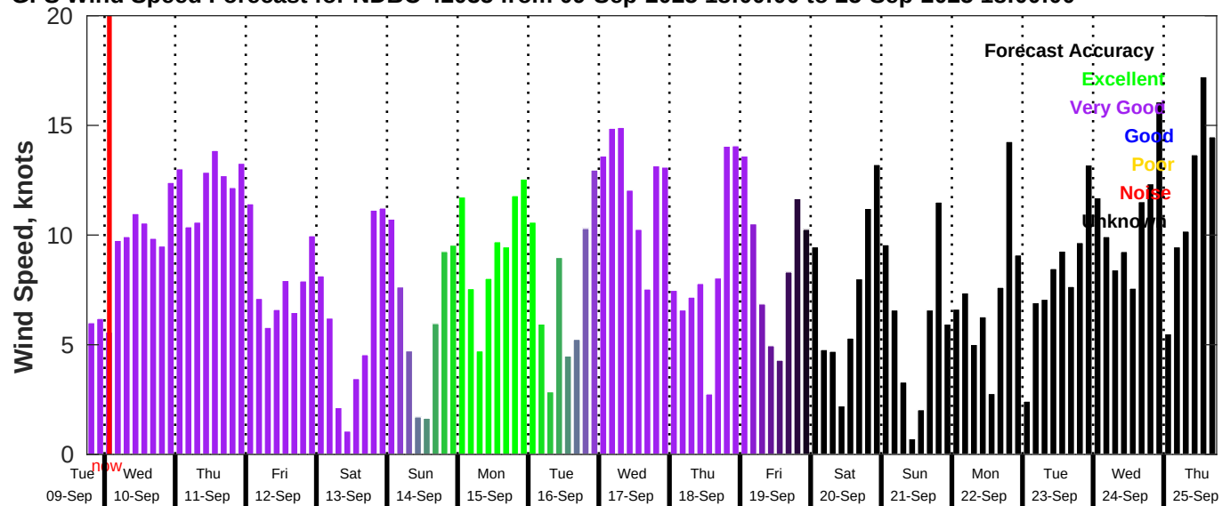
GFS Wind Speed Forecast for NDBC 42035 from 09-Sep-2025 18:00:00 to 25-Sep-2025 18:00:00
