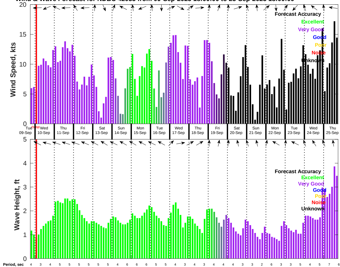
Wind & Wave Forecast for NDBC 42035 from 09-Sep-2025 18:00:00 to 25-Sep-2025 18:00:00
