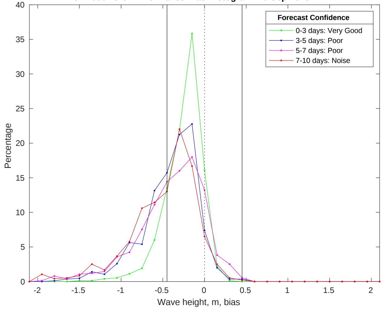
NDBC 42036 vs CMEMS Waves Bias Histogram: 10-Sep-2025
