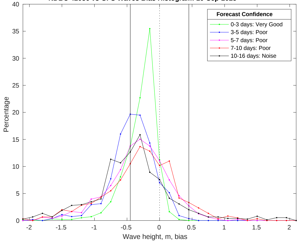
NDBC 42036 vs GFS Waves Bias Histogram: 10-Sep-2025
