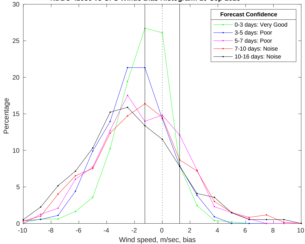
NDBC 42036 vs GFS Winds Bias Histogram: 10-Sep-2025
