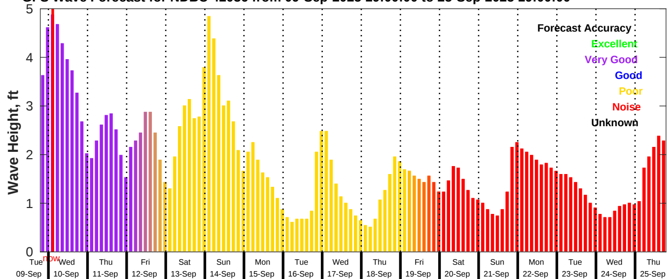
GFS Wave Forecast for NDBC 42036 from 09-Sep-2025 19:00:00 to 25-Sep-2025 19:00:00
