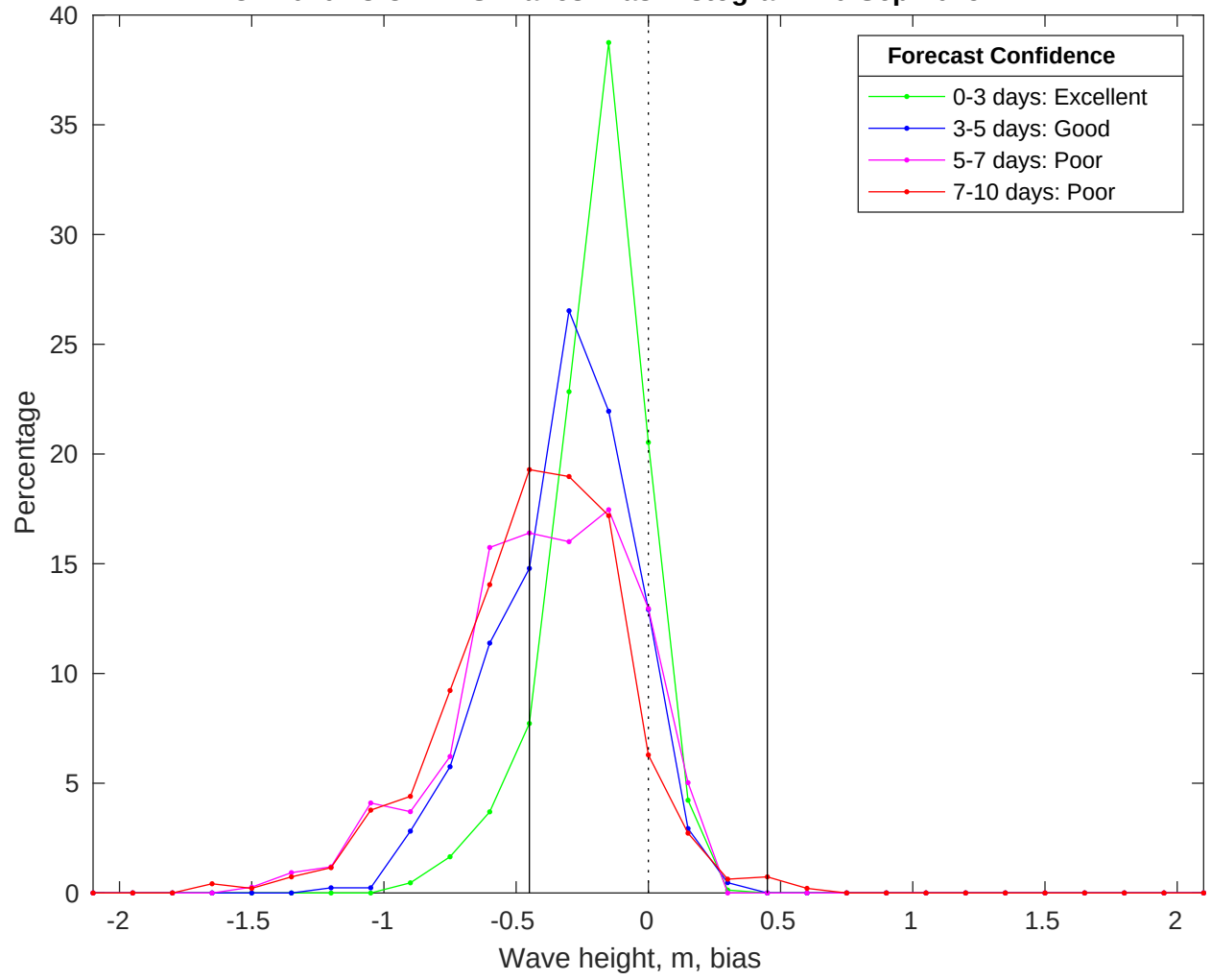
NDBC 42040 vs CMEMS Waves Bias Histogram: 10-Sep-2025
