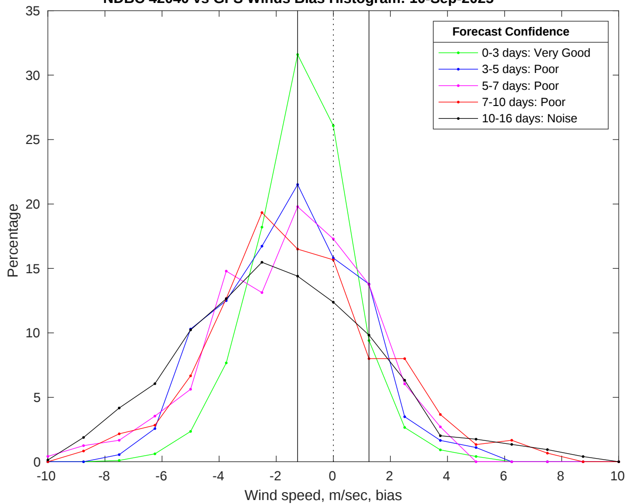
NDBC 42040 vs GFS Winds Bias Histogram: 10-Sep-2025
