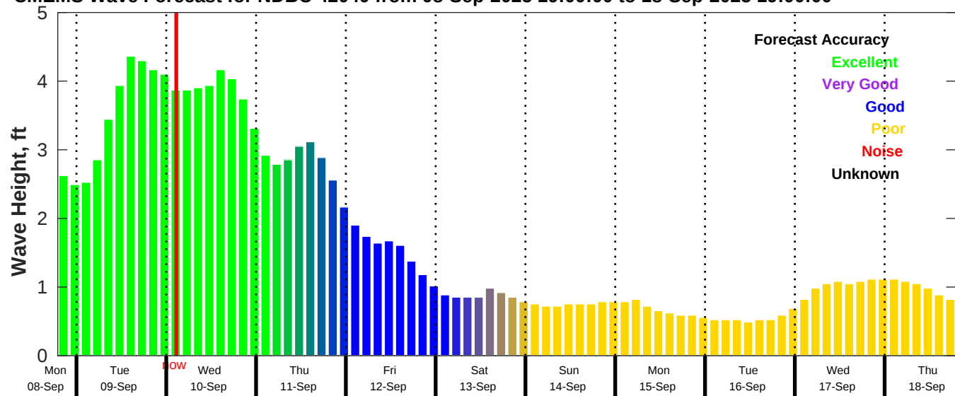
CMEMS Wave Forecast for NDBC 42040 from 08-Sep-2025 19:00:00 to 18-Sep-2025 19:00:00
